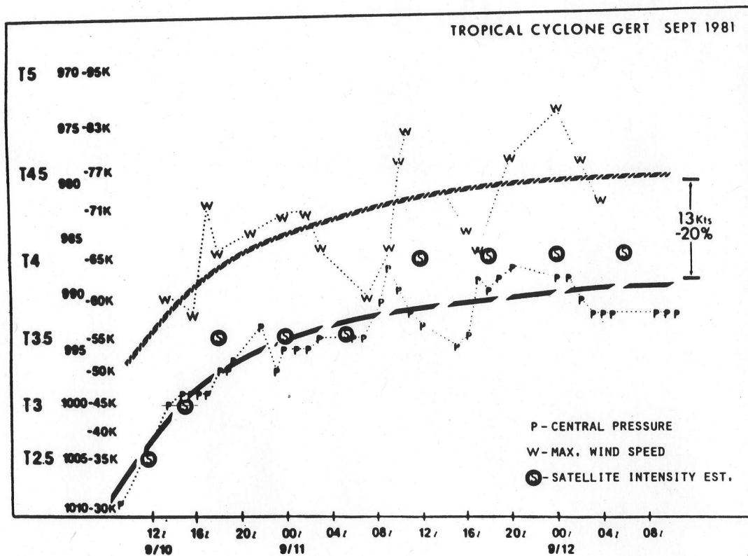
Fig. 15. A comparison of estimations of the intensity of tropical cyclone Gert, 1981. The maximum wind speed (W) and central pressure (P) estimates are from measurements taken on NOAA research aircraft. The satellite estimates (S) were made operationally at the Miami Satellite Field Services Station from EIR imagery.
