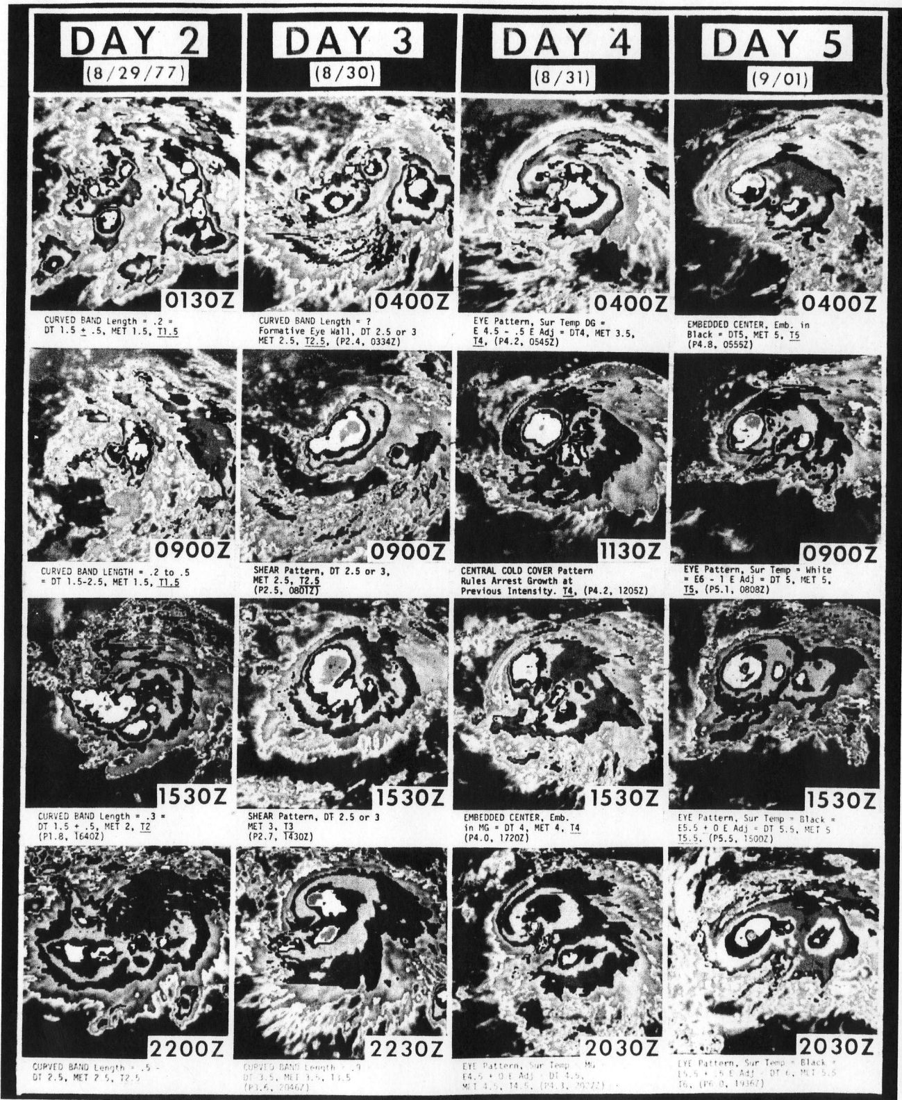
Fig. 12. Enhanced IR pictures taken at approximately 6-hour intervals are shown for 4 days in the life of hurricane Anita. The bottom two rows of pictures were taken at approximately the same time as the VIS pictures in Fig. 10.
