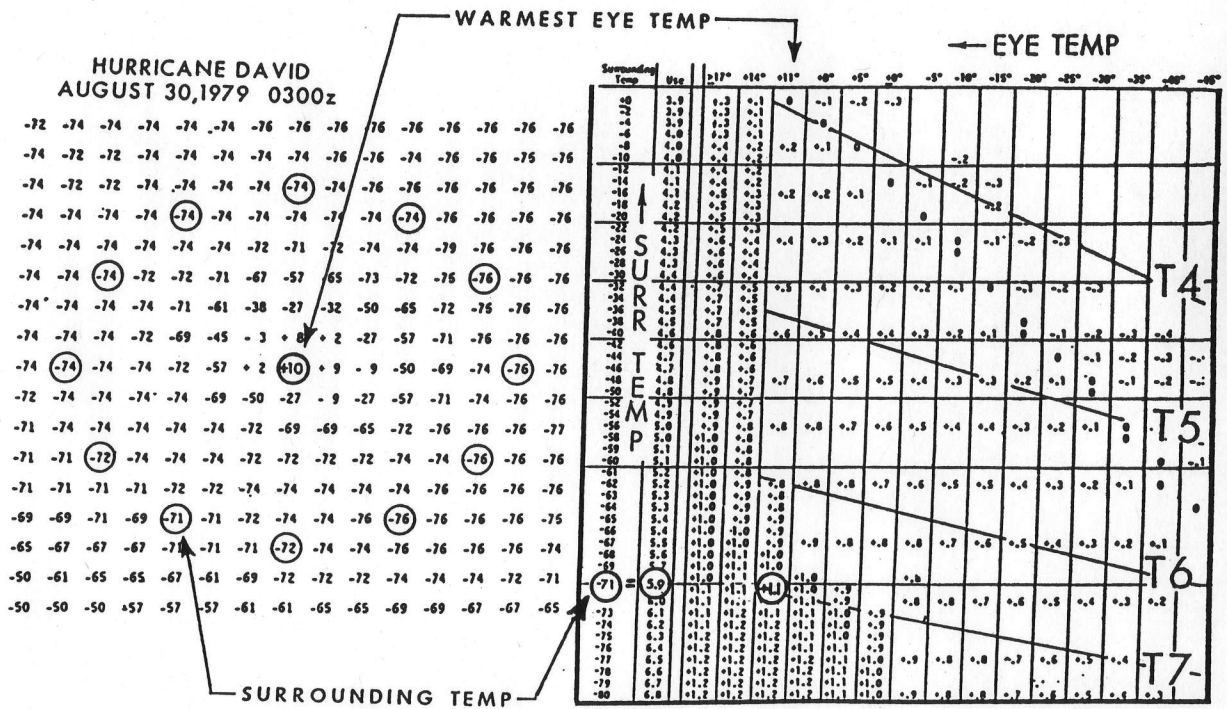
Fig. 9. Method for determining hurricane intensity from digital IR data. The digital printout on the left provides two temperature values which when entered in nomogram on the right result in an intensity estimate of T7. The surrounding temperature of -71°C contributes 5.9 while the relatively warm eye adds 1.1 to the T-number.
