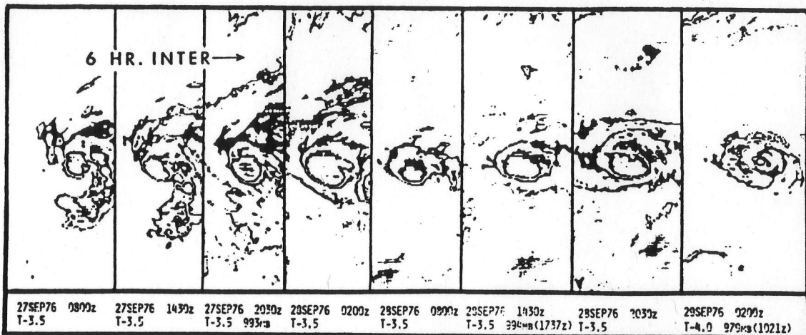
Fig. 7. Example of the life cycle of the Central Cold Cover (CCC). The central pressure of the storm stops falling when the CCC develops and the curved band begins to dissipate (Pictures at left). Pressure falls resume as the pattern redevelops (Pictures at right).
