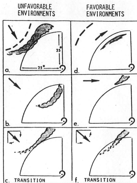
Fig. 13. Illustrations of environments that are unfavorable (left), favorable (right) for continued development of westward-moving tropical disturbances.
