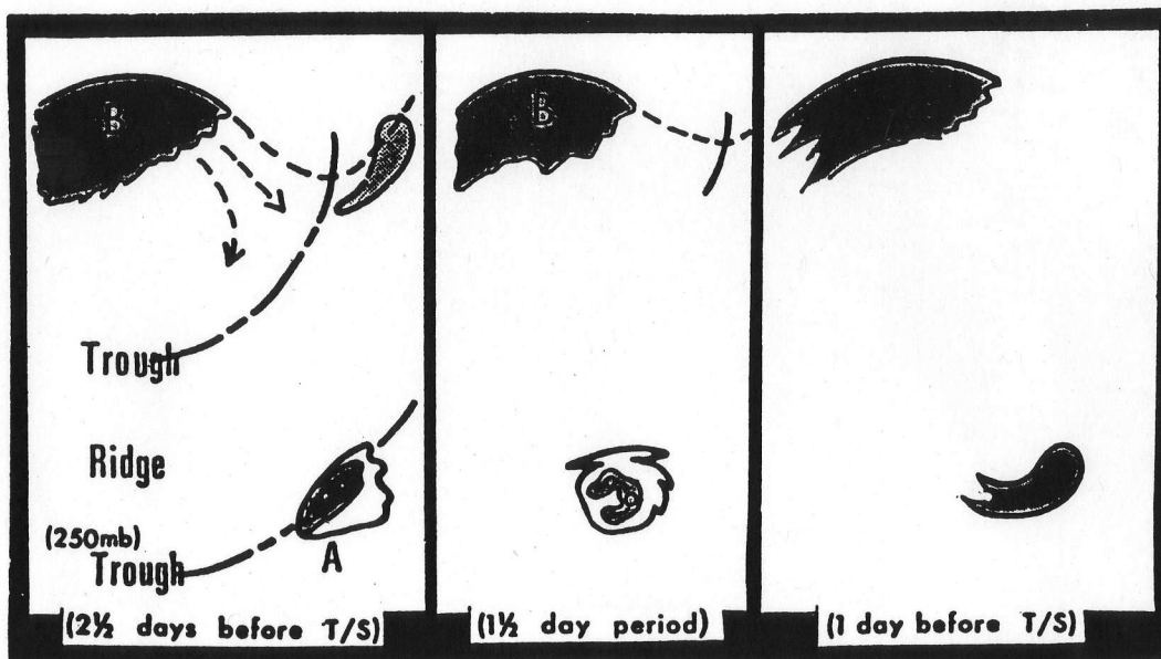
Fig. 14. Sequence of events associated with tropical cyclogenesis observed in most 1978 Atlantic storms. Cloud cluster is distorted by trough passages in left panel, then takes on a more circular pattern after trough passage (center), developing the curved band pattern about one day before tropical storm intensity is reached. After the trough passage, development is associated with anticyclonically curved banding or no banding to the northwest of the disturbance.
