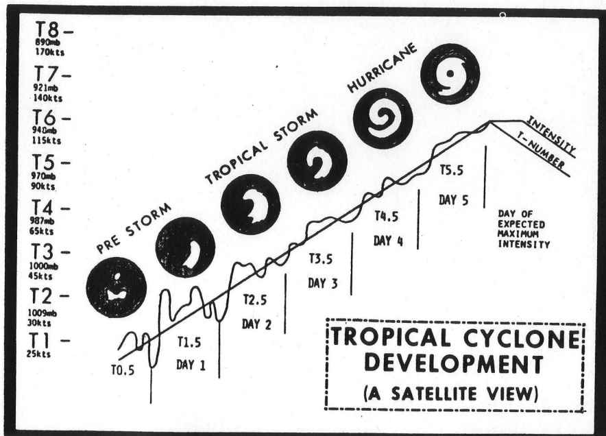
Fig. 1. Model of tropical cyclone development used in intensity analysis (curved band pattern type).
