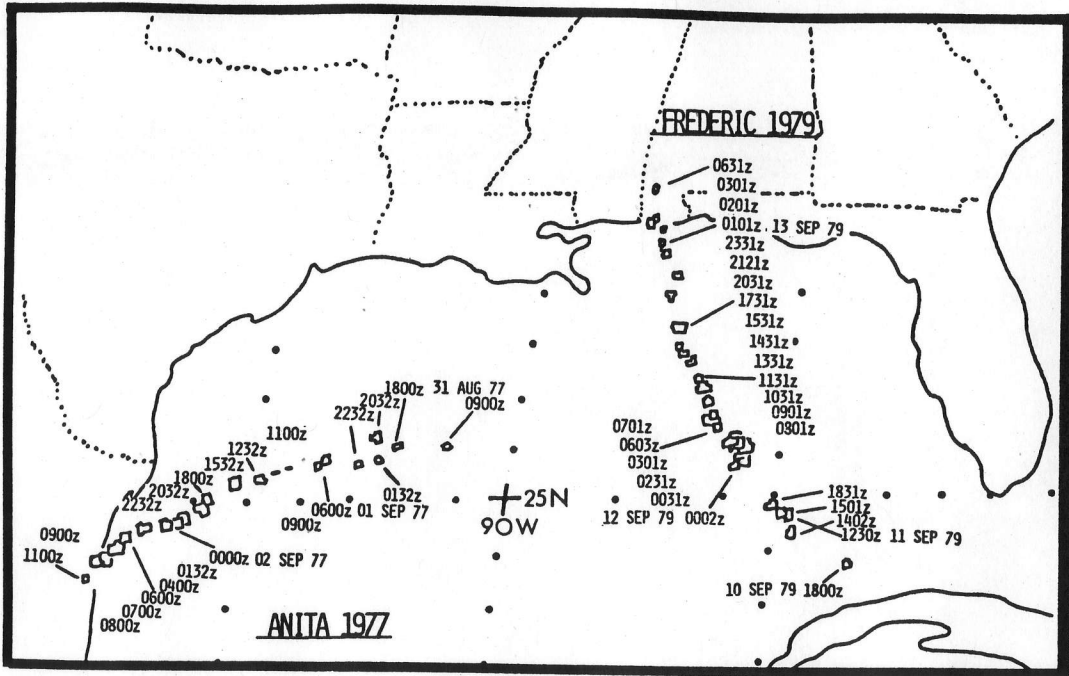
Figure 8. Tracks of hurricanes Anita and Frederic traced from the inner temperature contours of the eyes in enhanced IR pictures.
