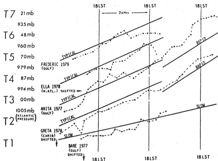
Figure 3. Plots of minimum central pressure for Atlantic hurricanes. Diagonal lines are modeled rates of intensity change used in analysis techniques.
